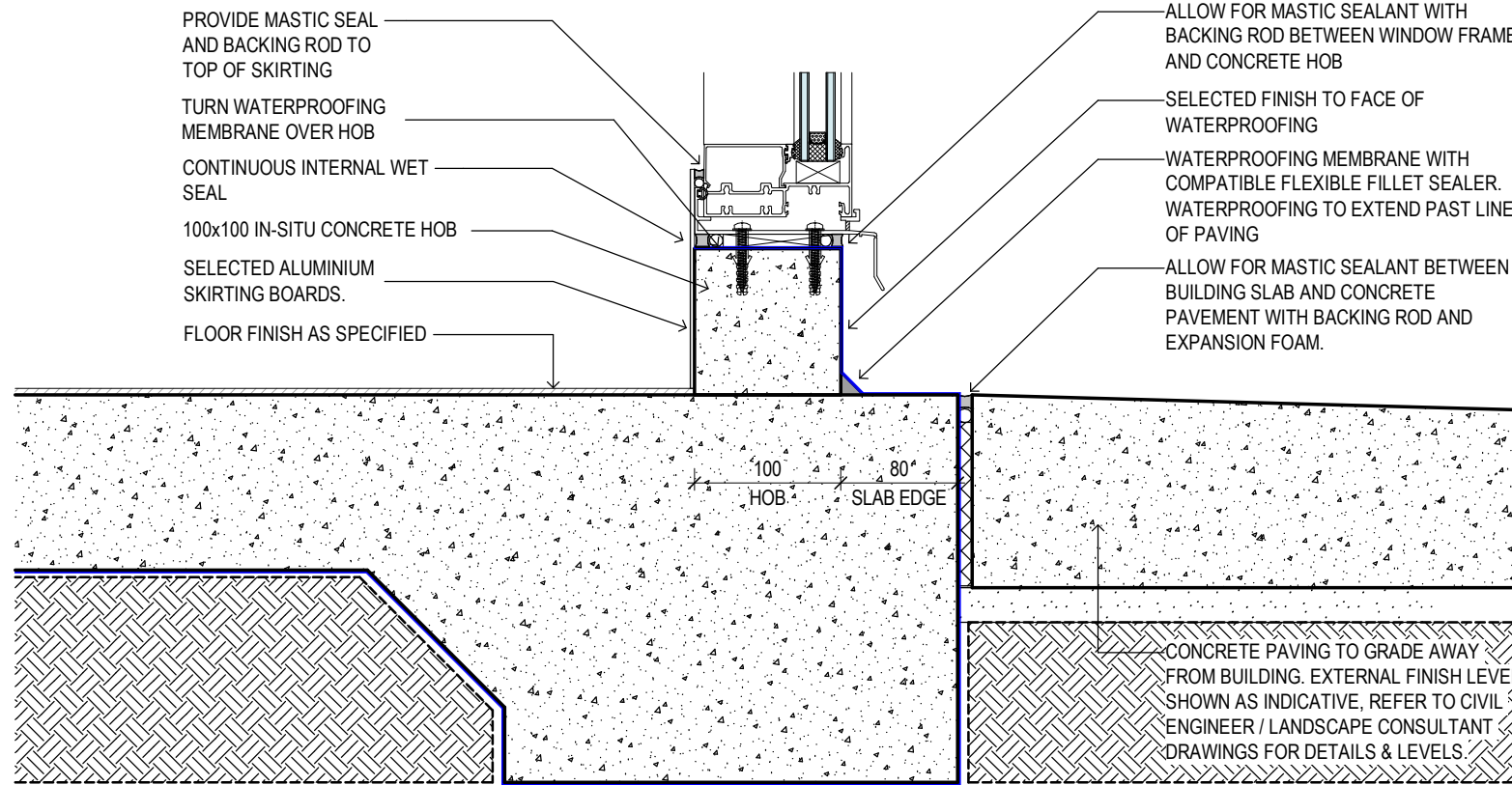
2 WINDOW UNIT ON CONCRETE HOB - BRICK VENEER INSET Scale 1:5
