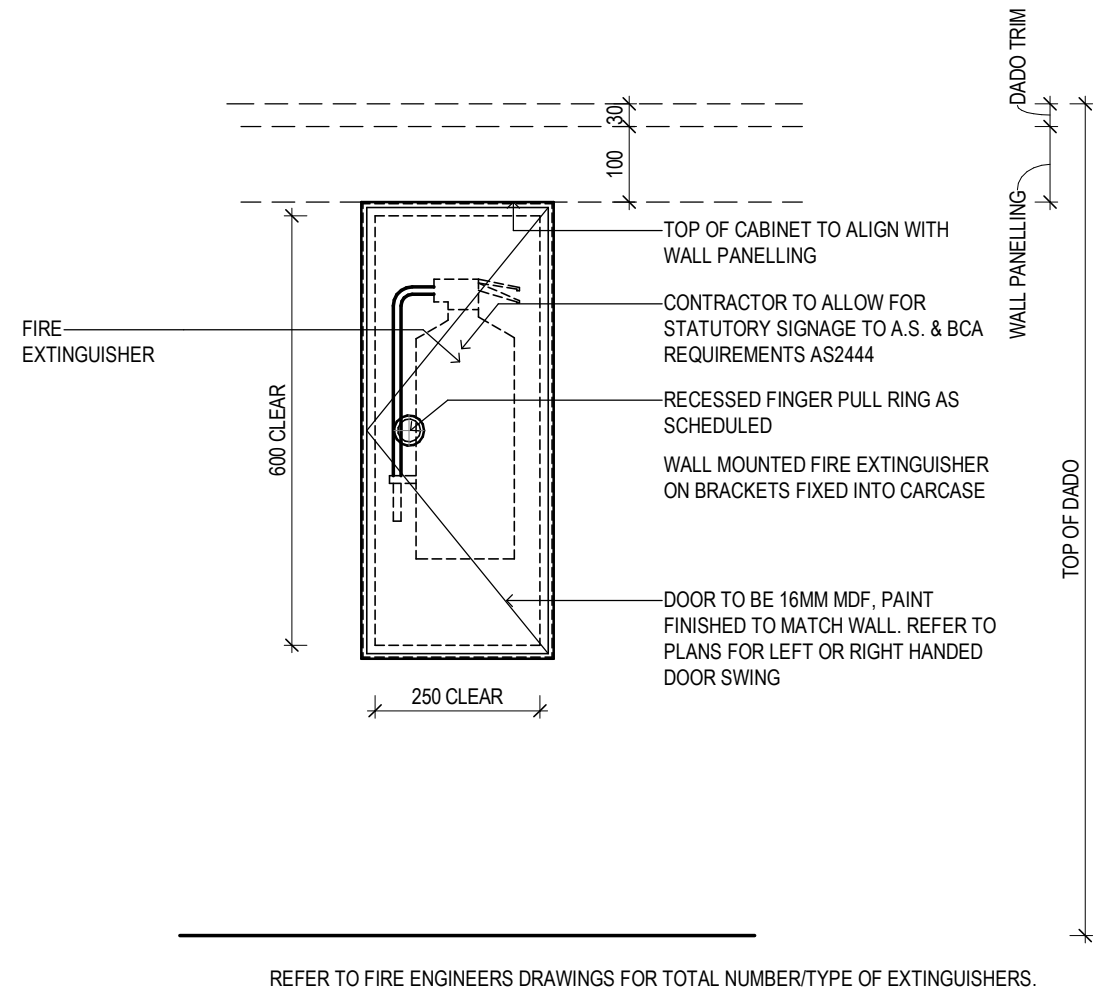
11 RECESSED FIRE EXTINGUISHER DETAIL ELEVATION - FE IN DADO Scale 1:10
