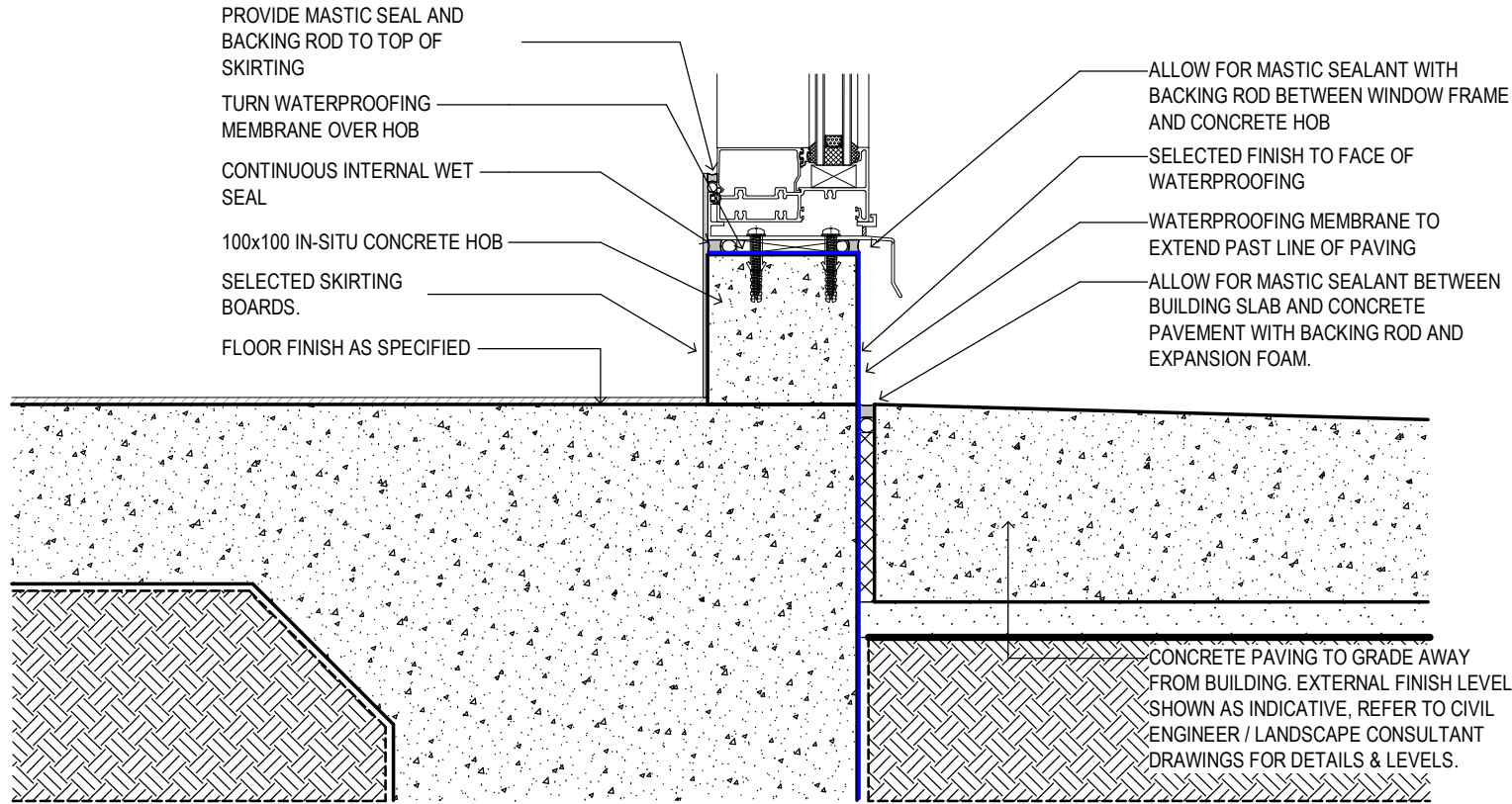
1 WINDOW UNIT ON CONCRETE HOB - SLAB EDGE Scale 1:5
