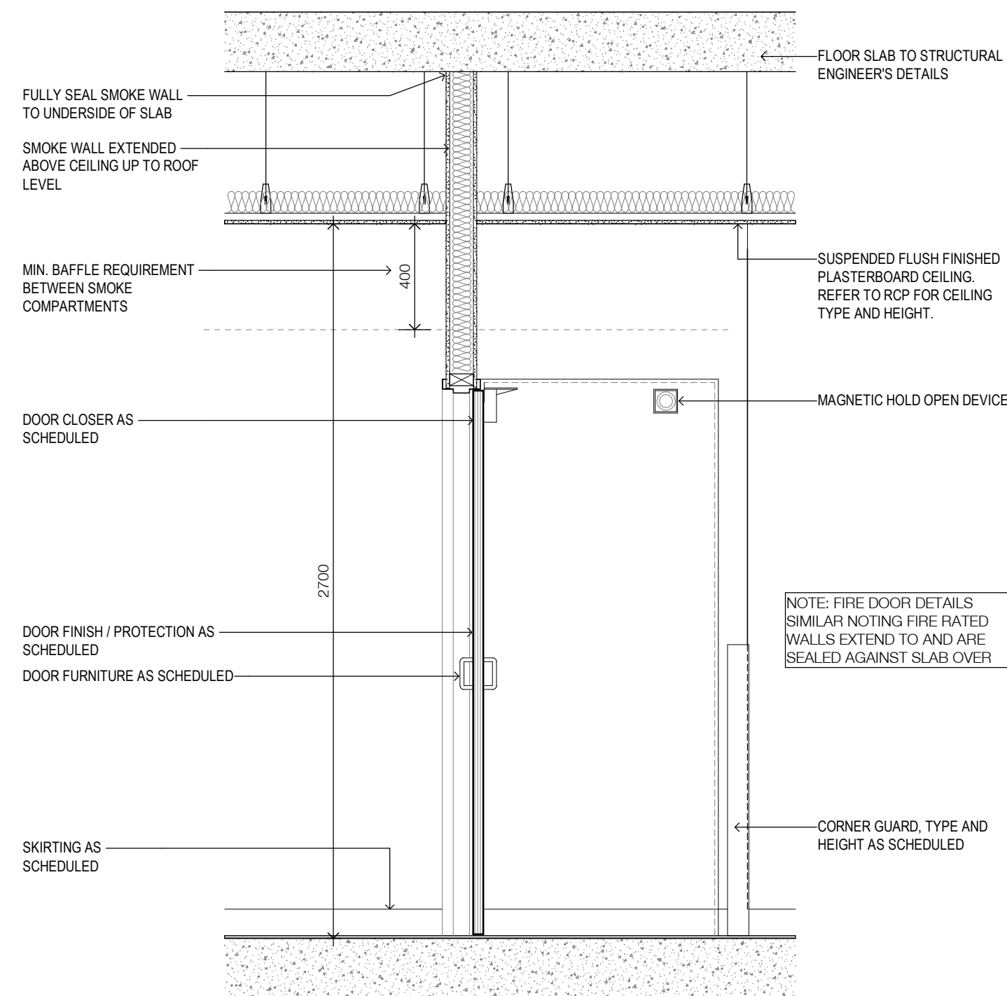
5 TYPICAL SMOKE DOOR SECTION - SLAB OVER Scale 1:20
