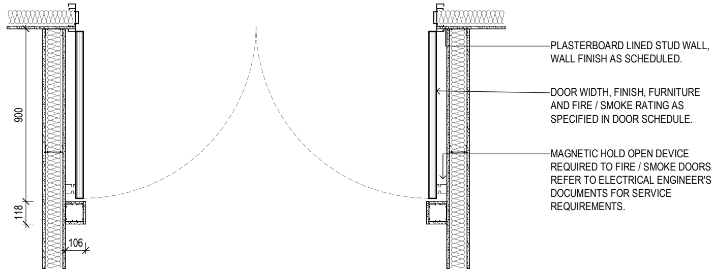
4 TYPICAL - SMOKE DOOR - PLAN Scale 1:20
