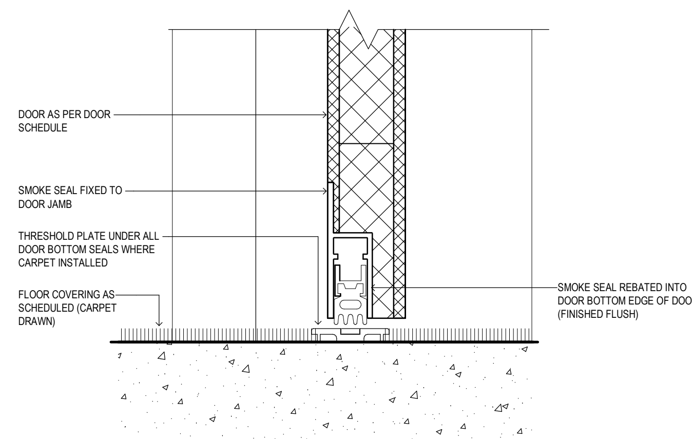
10 TYPICAL - SMOKE DOOR - SECTION DETAIL Scale 1:2
