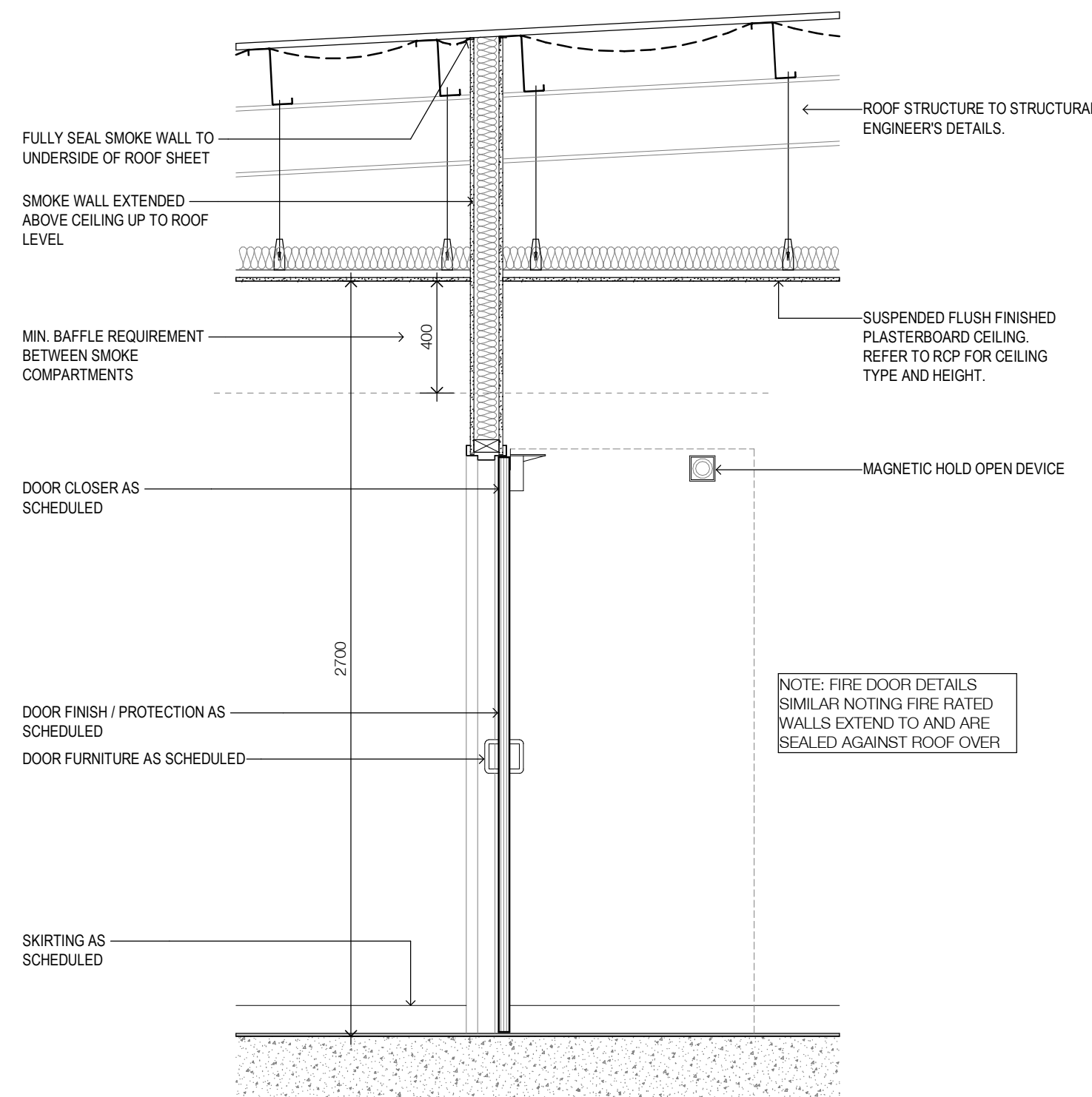
6 TYPICAL SMOKE DOOR SECTION - ROOF OVER Scale 1:20
