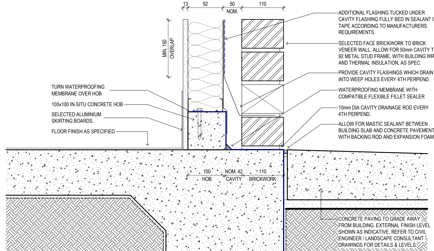
3 CONCRETE HOB TO BRICK VENEER Scale 1:5
