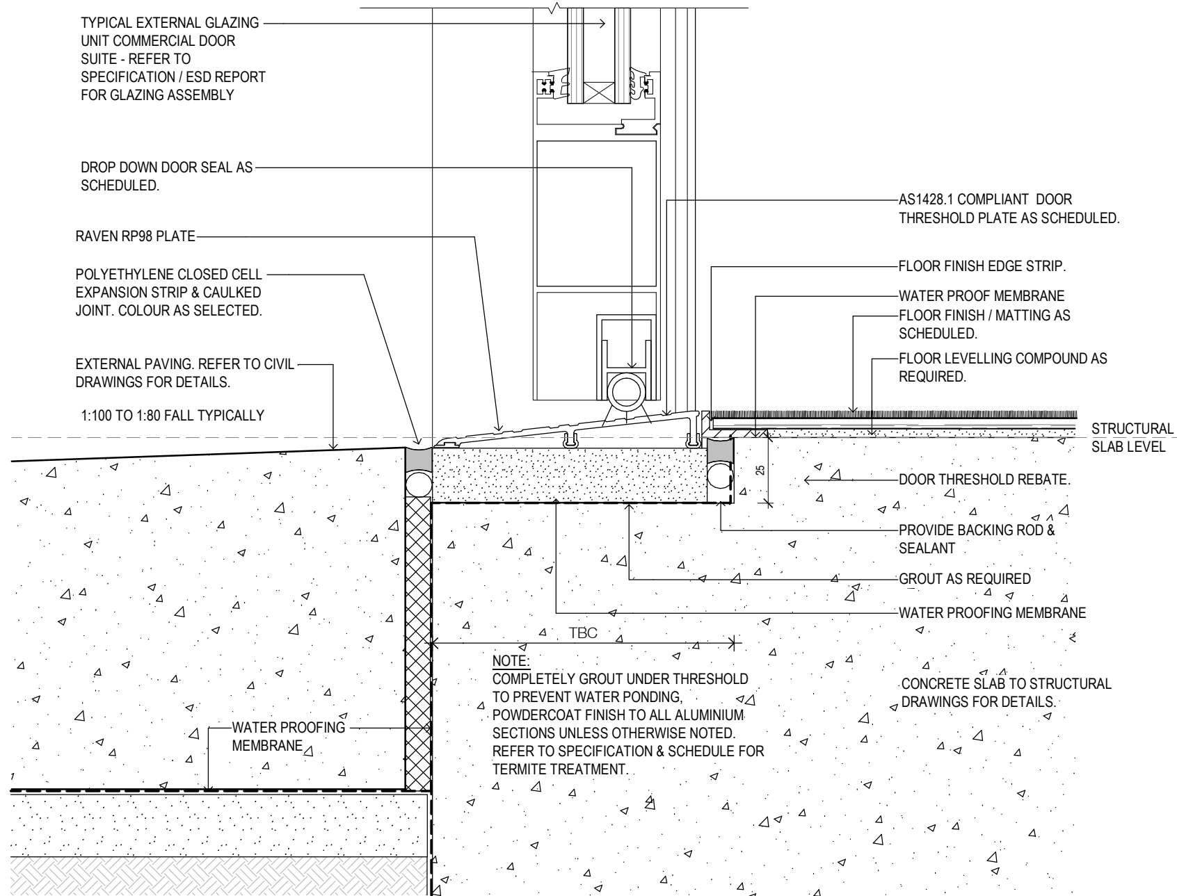
8 TYPICAL - EXTERNAL HINGE DOOR THRESHOLD - WITH THRESHOLD RAMP Scale 1:2
